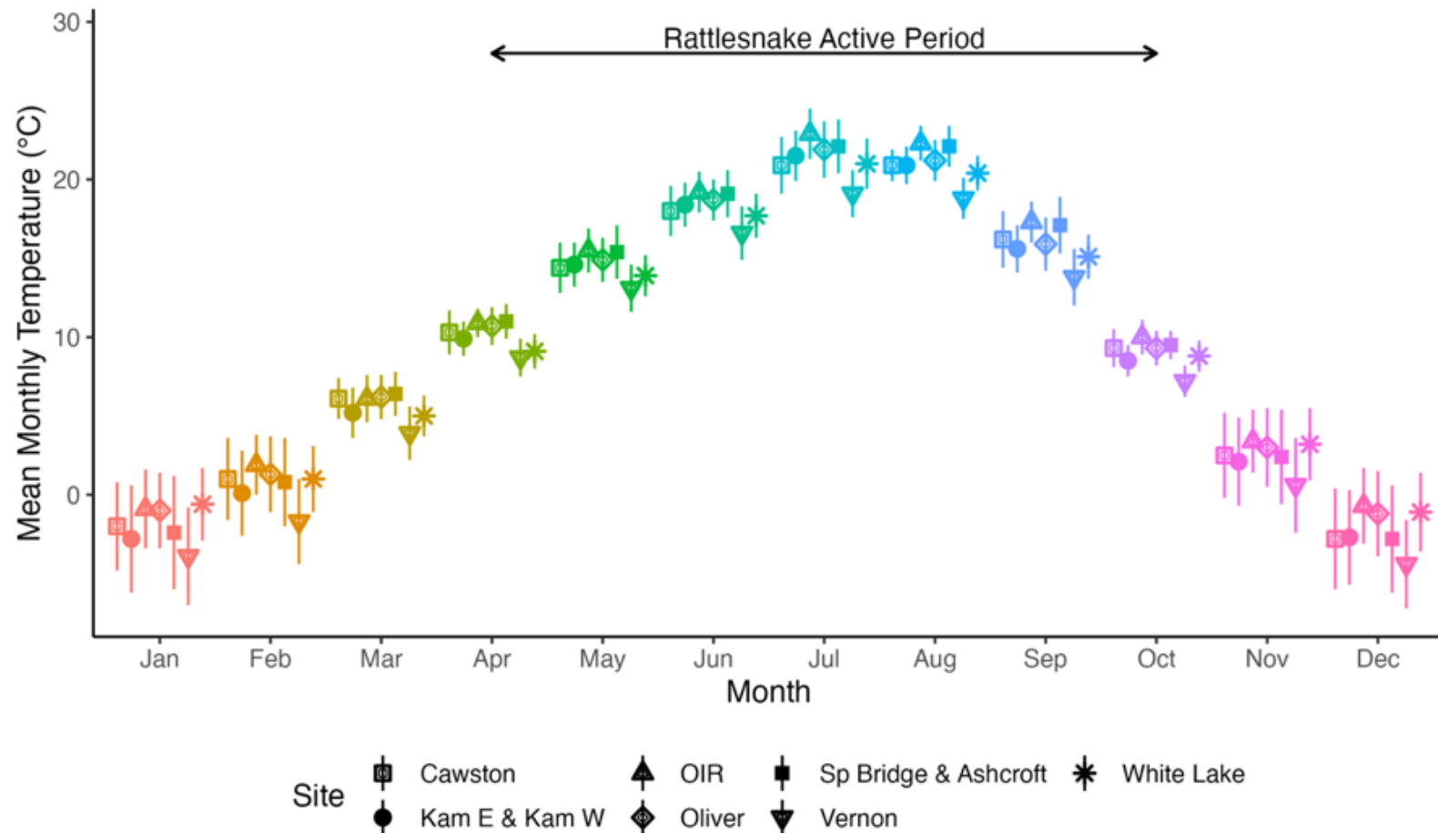
Figure 1.6. Historical 30-year (1981–2010) mean monthly temperatures (Environmental and Climate Change Canada 2023) across each of the nine study sites, using the closest available weather station (note that the same weather station was used for Kam E and Kam W, and for Spences Bridge and Ashcroft). Error bars represent \pm 1 standard deviation. Data from Environment and Climate Change Canada (2023). Site abbreviations: OIR = Osoyoos Indian Reserve; Kam E = Kam East; Kam W = Kam West; Sp Bridge = Spences Bridge. Actual weather station names: Cawston = Keremeos 2; Kam E & Kam W = Kamloops A; OIR = Osoyoos CS; Oliver = Oliver; Sp Bridge & Ashcroft = Spences Bridge Nicola; Vernon = Vernon Coldstream Ranch; White Lake = Penticton A.
