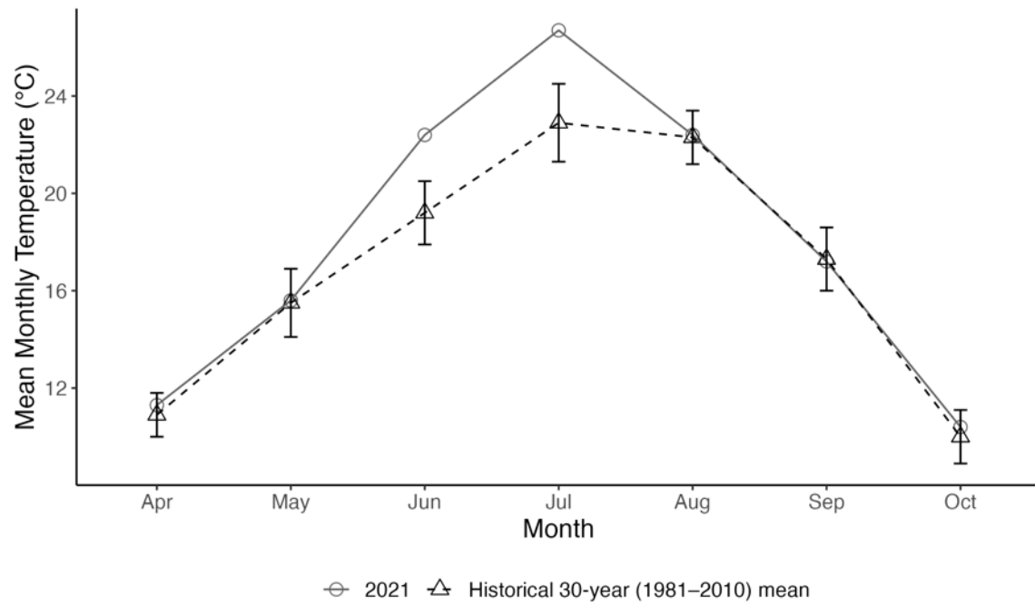
Figure 1.3. Mean monthly temperatures (°C) in Osoyoos, British Columbia, in 2021 (circles) compared to the historical 30-year mean (1981–2010; triangles) during the months of April through October (rattlesnake active season). Values measured at the Osoyoos weather station (49.03° N, 119.44° W). Data from Environment and Climate Change Canada (2023).
