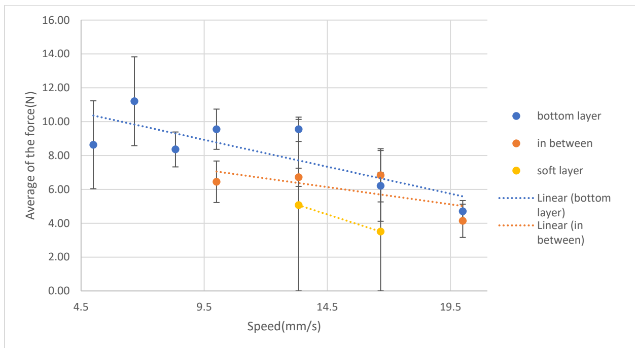
Figure 25. Average of the means of the plateau for each trial in three layers plotted as function of the speed (mm/s). Snow samples were collected from Sun Peaks area.
