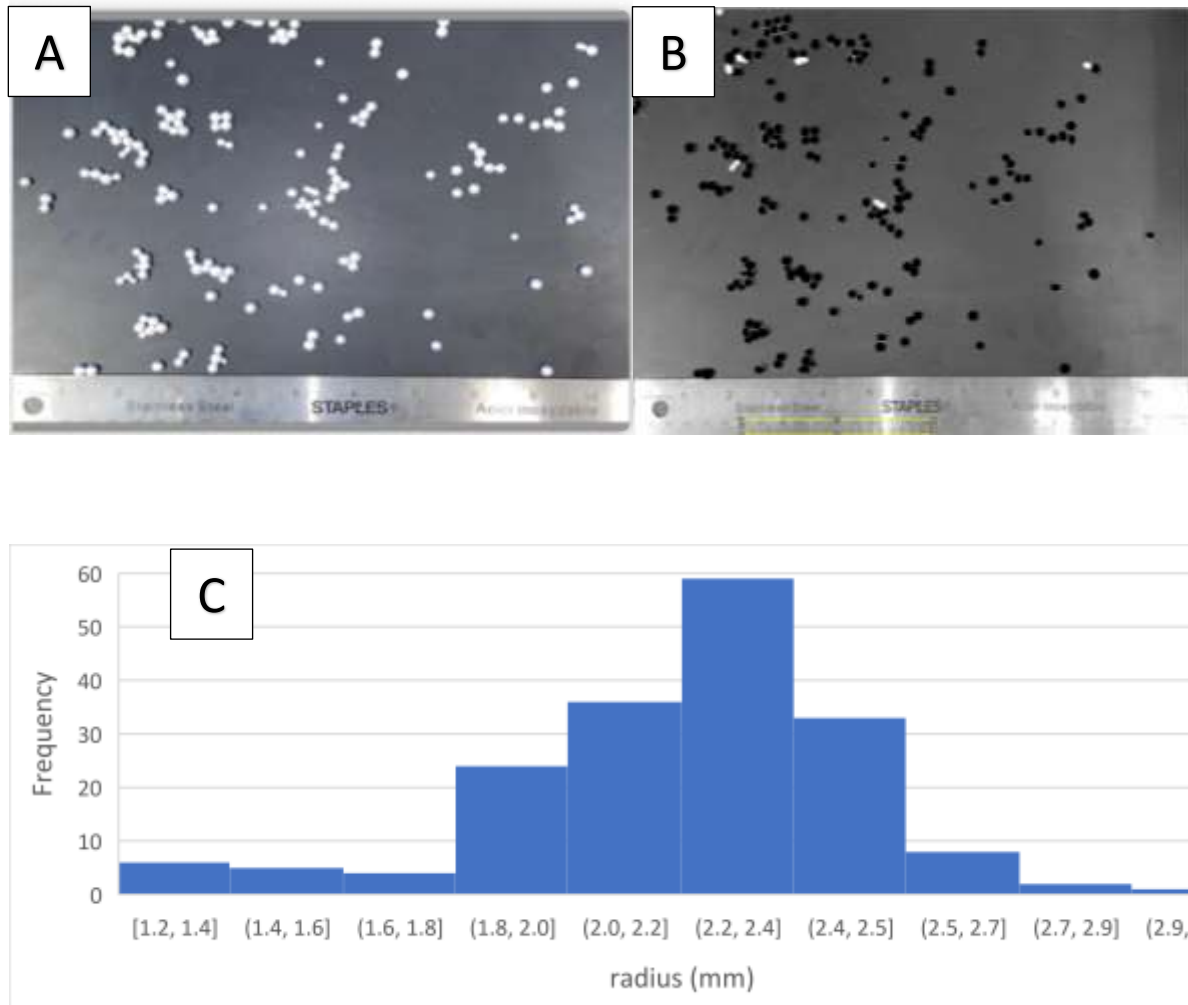
Figure 3 A. Raw image of the polystyrene beads taken using phone camera. The ruler was used as reference for the measurements. B. Image of the polystyrene particles assumed circular obtained ImageJ. C. Distribution of the polystyrene particles size centered with a peak at 2.3 mm radius.
