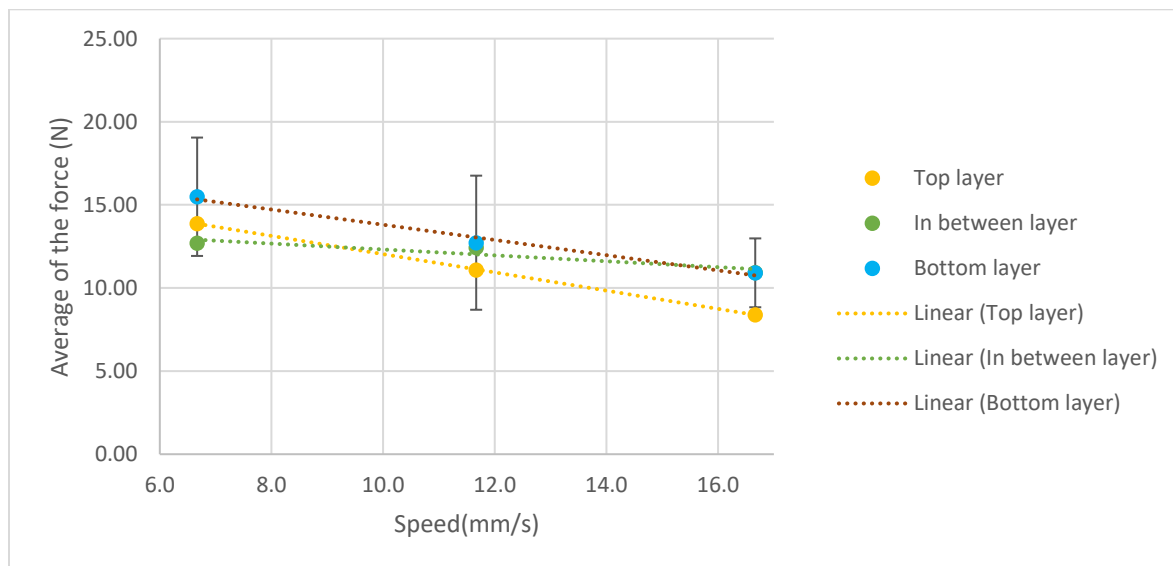
Figure 24. Average of the means of the plateau for each trial in three layers plotted as function of the speed (mm/s). Snow samples were collected from Stake Lake area.
