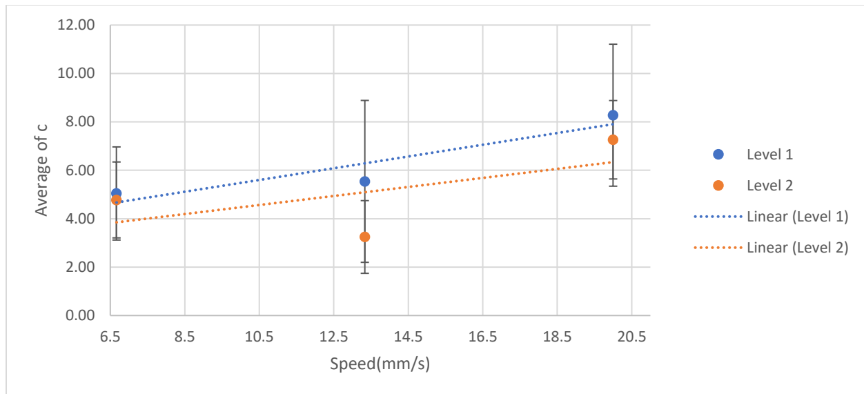
Figure 33. Horizontal measurements of the wet sand moisten at 15%. The blue series represents data of blade insertion at level 1 of the sand box; orange series represents data taken at level 2.
