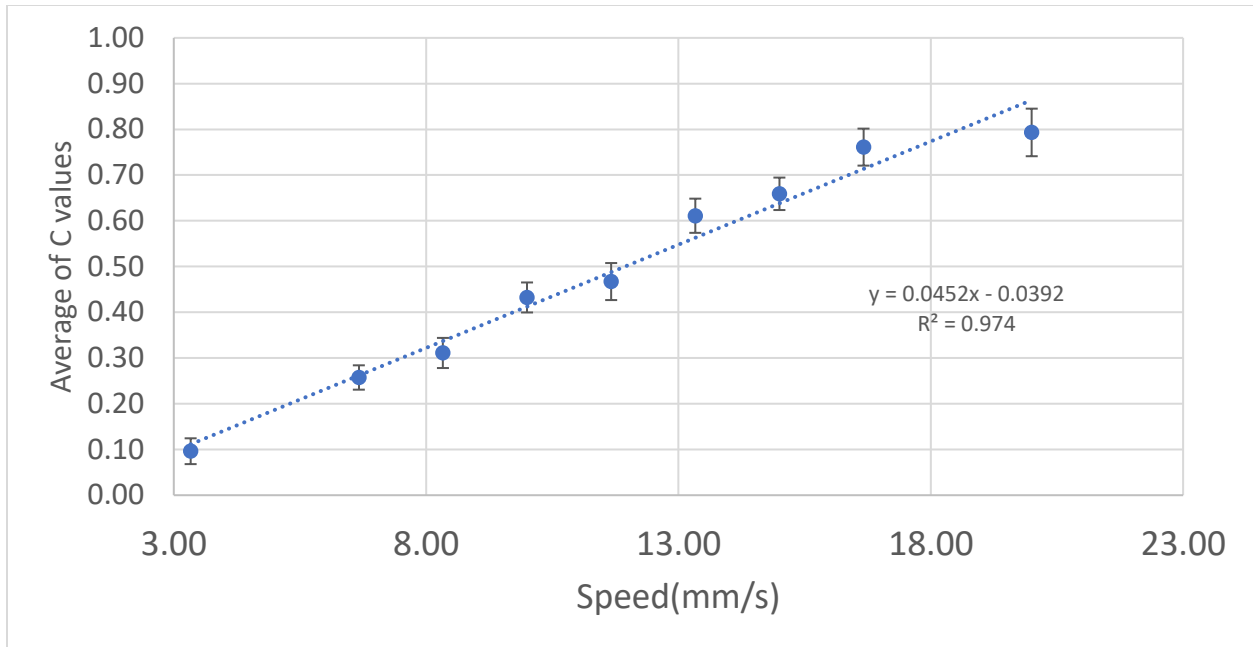
Figure 7. Average of c from F = F_0 e^{ct+\beta} plotted against the speed (mm/s) from the dry sand measurements using the aluminum blade ( 11.50 \pm 0.10 cm length, and 1.04 \pm 0.01 mm thickness). The dotted line is a linear fit to the data.
