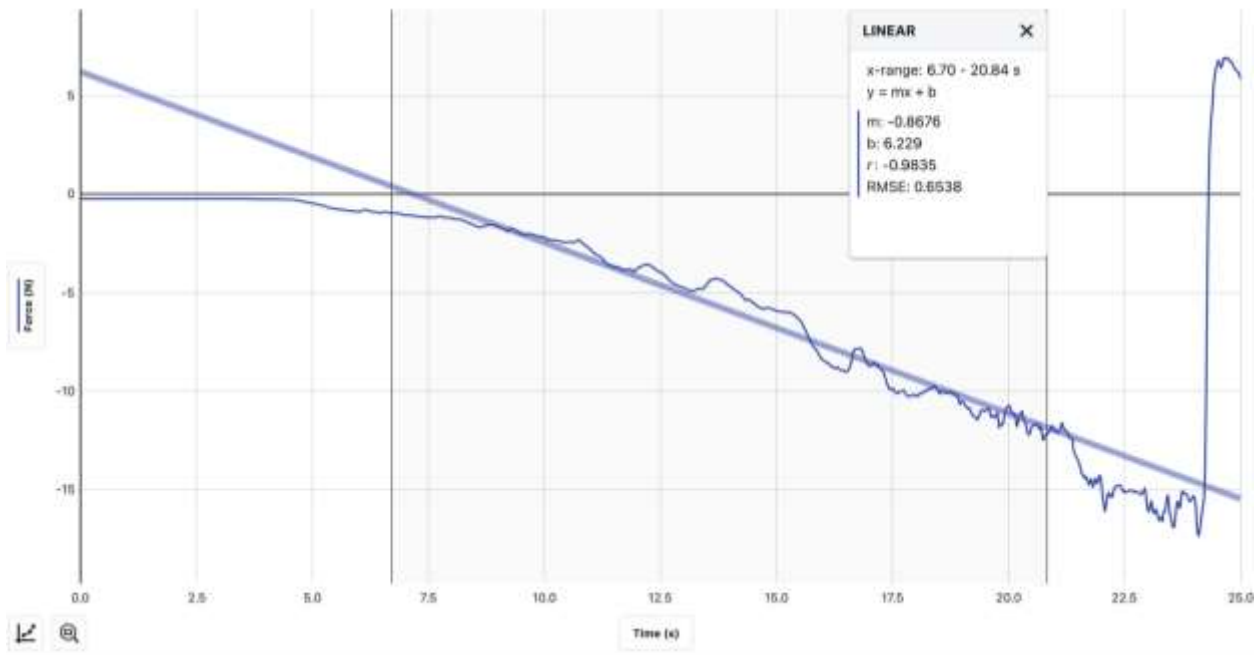
Figure 11. The resistive force (N) as a function of the time(s) at a speed of 3.33mm/s, a vertical penetration of an aluminum blade with a length equal to 11.5 \pm 0.10 cm, and a thickness of 1.04 \pm 0.01 mm. The time between 0 to 5s, the graph is matching the 0 N force line as the blade was not inserted yet. After 5s the blade starts penetrating the granular material until time equal to 24s when it stops and goes back to the initial position.
