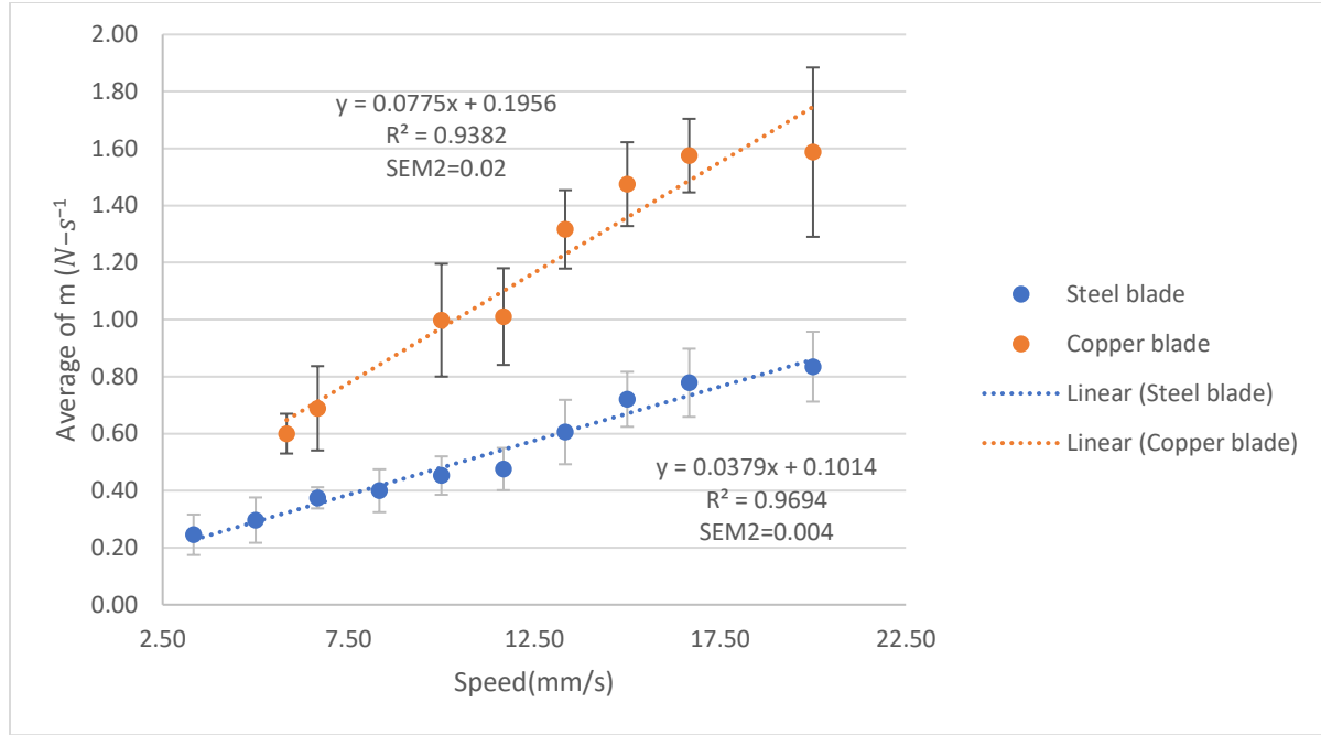
Figure 13. Measurements of \bar{m} ( Ns^{-1} ) from F = \mathbf{m}t + \mathbf{b} performed in the polystyrene, and by using the steel blade and the long copper blade. The dotted line is straight line fits to the data.
