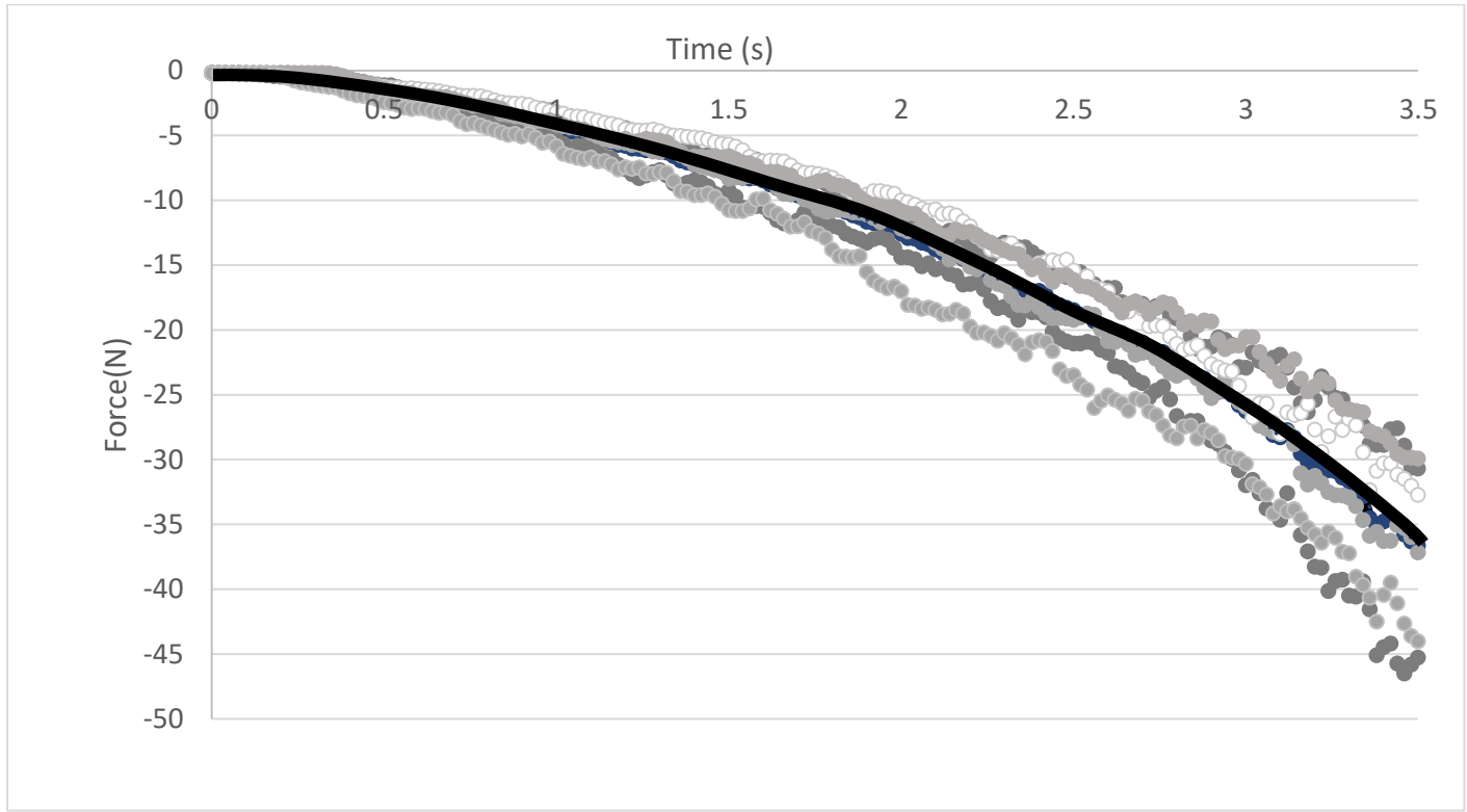
Figure 6. For six different runs, this figure exhibits the measured force as the blade is inserted at 11.7 mm/s. The solid line is the average of all runs; the average of c value is 0.56 \pm 0.08 \text{ s}^{-1} . All trials display similar exponential behavior.
