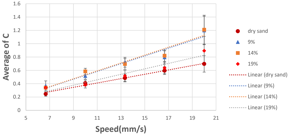
Figure 15. Results of wet sand measurements moisture at 9%, 14%, and 19%. Average of c ( s^{-1} ) was calculated based on the c values in figure 12 and plotted as function as the speed (mm/s). the linear fit of the data was added, as a guide for the eye, to follow where most of the same percentage of data is located.
