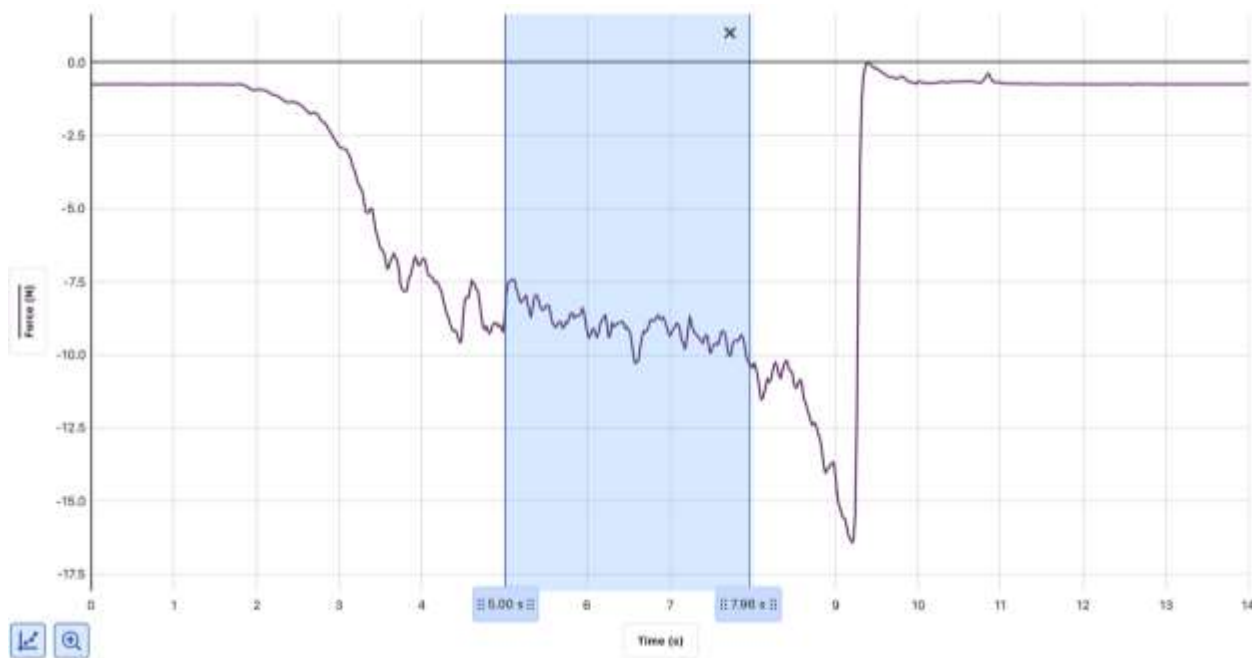
Figure 18 Example of raw data of the blade hardness gauge inserted at a speed of 6.7mm/s into a hard layer of the snow sample. The type of blade was the short copper blade, 20.00 \pm 0.10\text{mm} , length, 14.44 \pm 0.10\text{mm} , thickness. The purple line indicates the fluctuations of the force in the snow sample, and the blue highlighted area is where the plateau was detected. The blade starts penetrating the snow sample at approximately 2s, and it goes back to the initial position at 9.3s.
