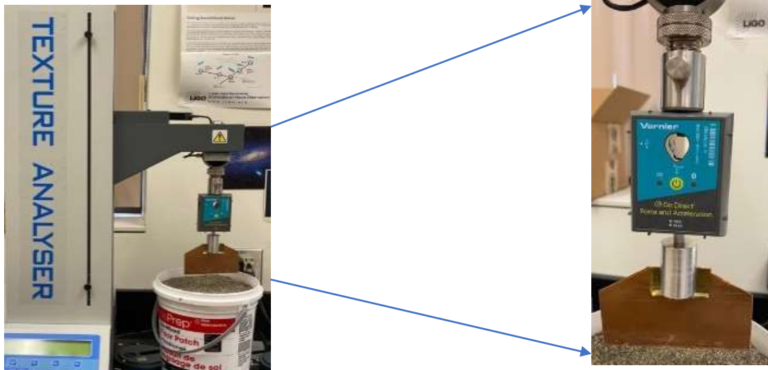
Figure 4. a) The Texture Analyser used to provide constant vertical speed. b) The force meter used to measure the vertical force on the blade.
