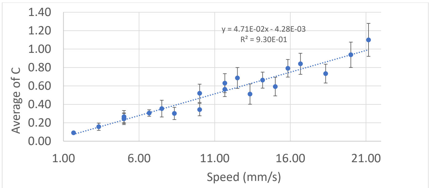
Figure 8. Values of \bar{c} plotted as a function of the speed (mm/s). The measurements were performed by means of the short copper blade in the dry sand. The dashed line in the inset is the linear fit of this data.
