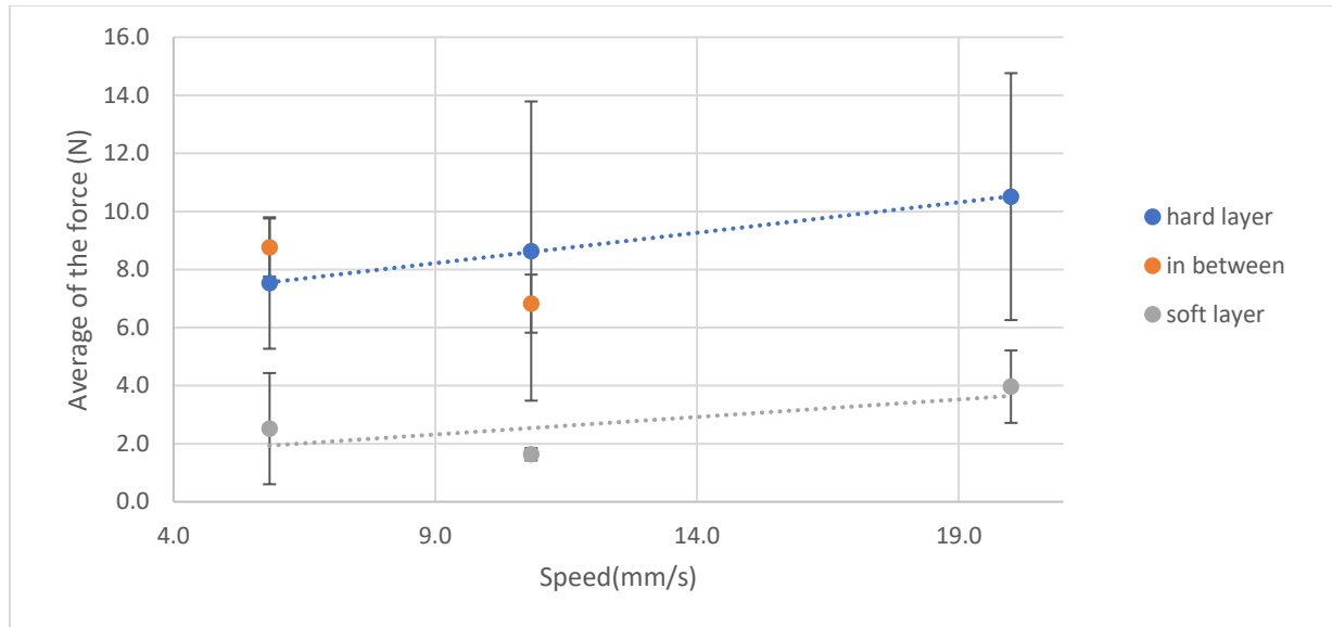
Figure 20. Average of the means of the plateau for each trial in three layers of the snow sample collected from the second site around the campus. The measurements were carried out at a speed between 5.8mm/s and 20 mm/s.
