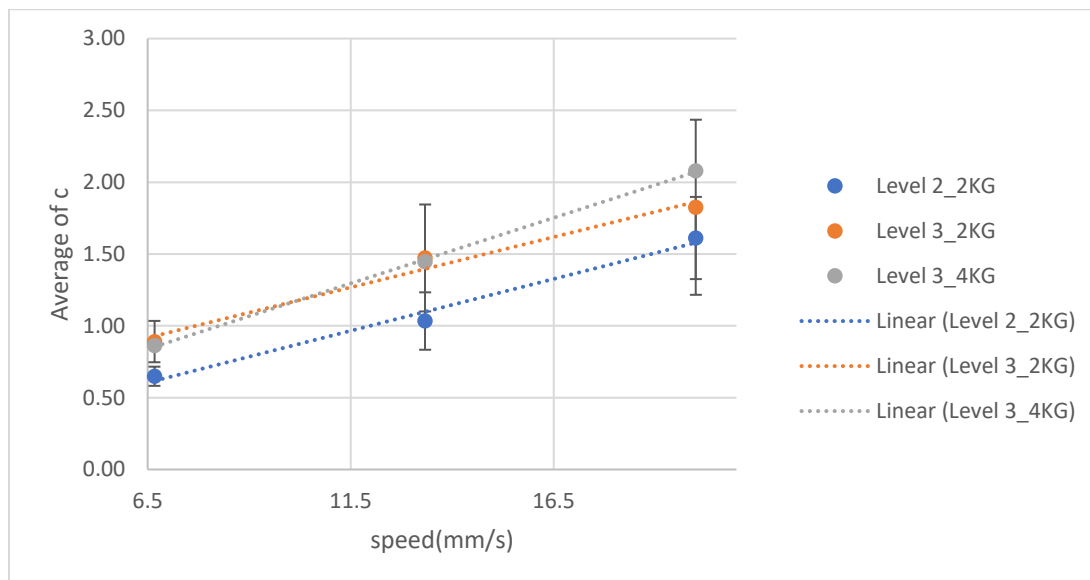
Figure 29. Horizontal measurements of the polystyrene. The blue series represents data of blade insertion at level 2 of the box with 2kg weight added on the top; orange series represents data taken at level 3 with a compaction of 2kg on top. Lastly, grey series shows data taken at level 3 with a weight of 4 kg on top of the box. The dashed line in the inset is the linear fit of this data.
