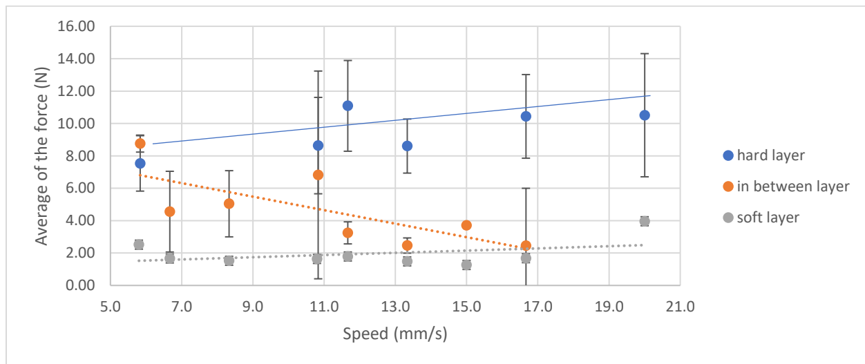
Figure 23. Average of the means of the plateau for each trial in three layers of the snow sample collected from sites around the campus. The measurements were carried out at a speed between 5.8mm/s and 20mm/s.
