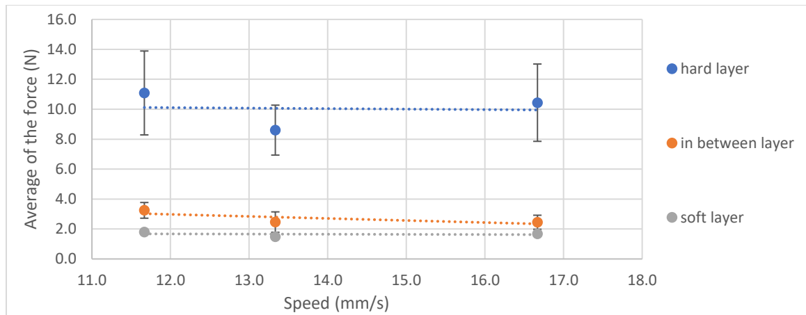
Figure 21. Average of the means of the plateau for each trial in three layers of the snow sample collected from the third site around the campus. The measurements were carried out at a speed between 11.7mm/s, 13.3mm/s, and 16.7mm/s.
