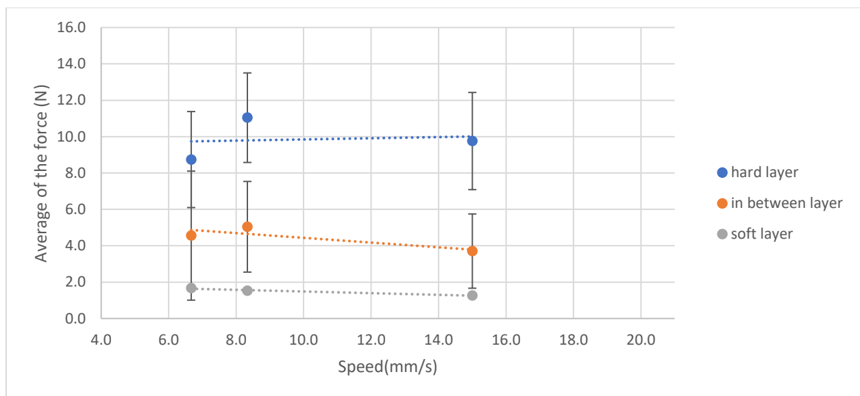
Figure 22. Average of the means of the plateau for each trial in three layers of the snow sample collected from site number 4 around the campus. The measurements were carried out at a speed between 6.7mm/s, 8.3mm/s, and 15mm/s.
