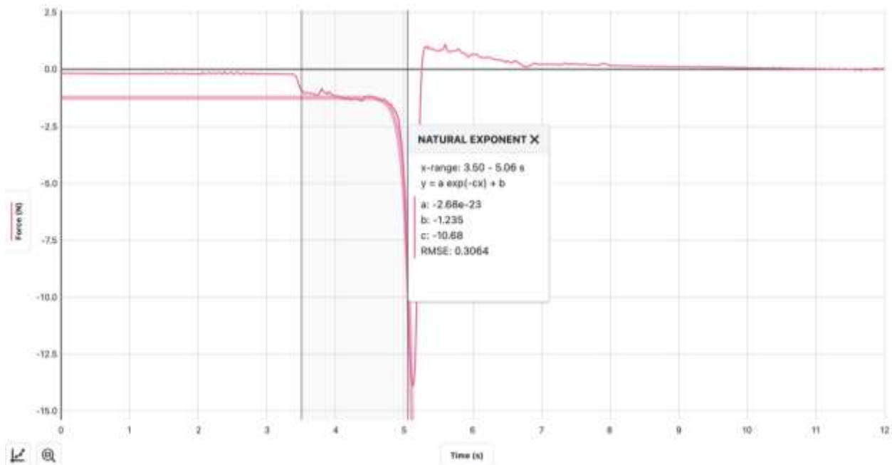
Figure 31. Raw data of wet sand containing 15% of moisture measured using Vernier force meter. The graph represents force versus time for a speed equal to 20mm/s, where the blade was inserted matching level 1 in the box horizontally. The time between 0 to 3.5s, the graph is matching the 0 N force line as the blade was not inserted yet (with some noises at the beginning of the insertion and at the end due to the blade was in contact with the cover of the box). After 3.5s the blade starts penetrating the sand until time equal to 5.1s when it stops and goes back to the initial position.
