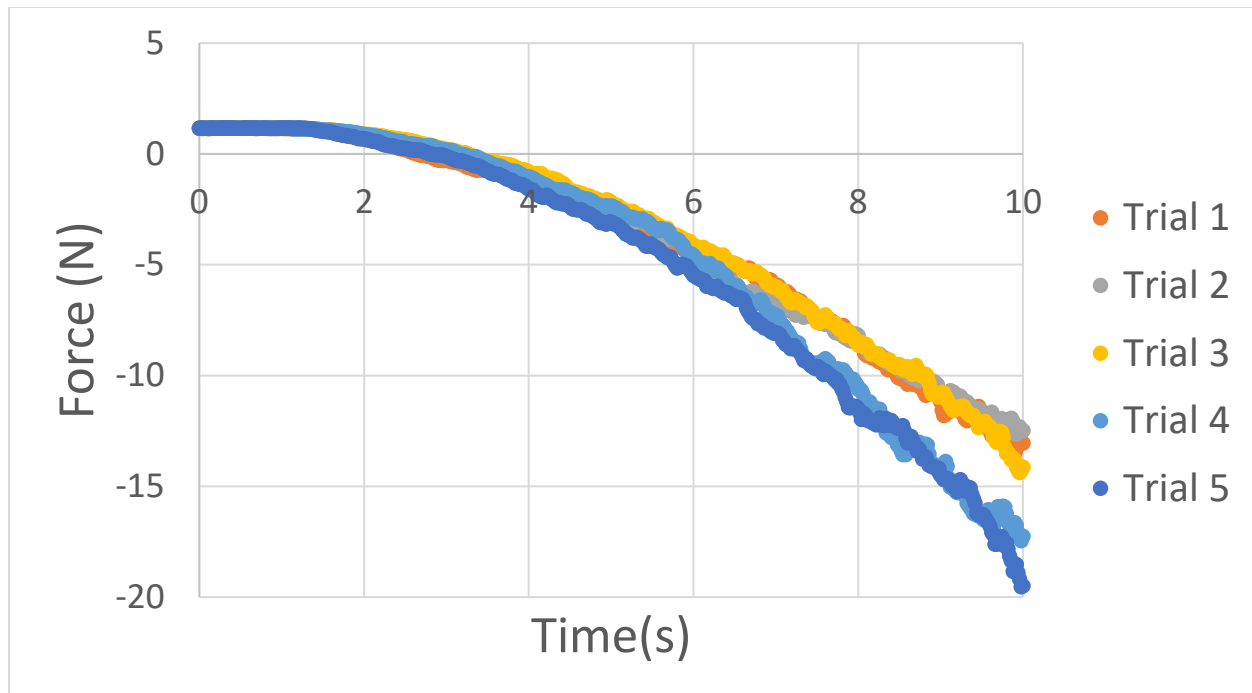
Figure 32. For five different runs, this figure shows the measured force as the blade is inserted at 20 mm/s into wet sand moisten at 15%. All trials display similar behavior.
