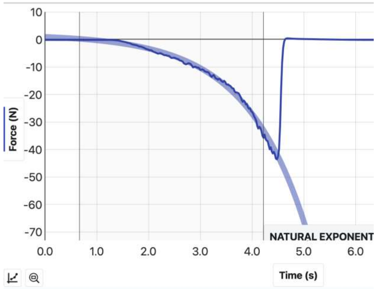
Figure 5. Data from the lab evaluations in dry sand measured using Vernier force meter. The type of blade was the short copper blade, 12 \pm 0.10 cm length, and 1.22 \pm 0.07 mm in thickness. The graph represents force versus time for a speed equal to 12.5 mm/s. The solid blue line indicates the fluctuations of the force in the granular material, and the light blue line is an exponential fit to the
