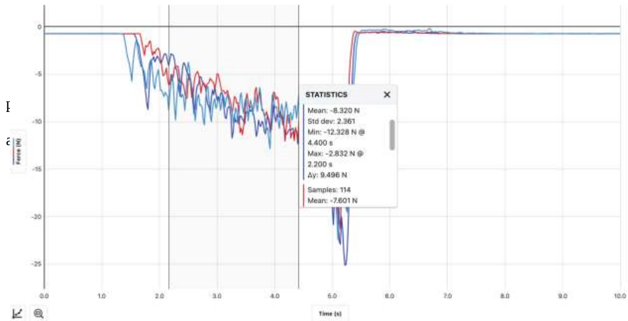
Figure 19 For three different trials, this figure exhibits the average of the plateau of the three trials displayed in three different colours using the Vernier software. the speed of penetration is 13.3mm/s into the hard layer of the snow sample collected from campus area.
