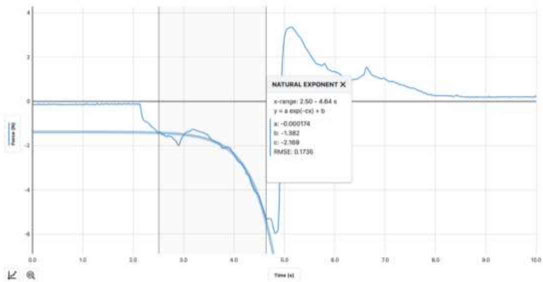
Figure 27. Data from the lab evaluations in polystyrene measured using Vernier force meter. The graph exhibits force versus time for a speed equal to 20mm/s, where the blade was inserted matching level 3 in the box, and with 2kg weight added on top. The light blue line indicates the fluctuations of the force in the polystyrene, and the solid blue line is an exponential fit to the data curve. The blade starts going inside the polystyrene at approximately 2.3s, and it goes back to the initial position at 5s.
