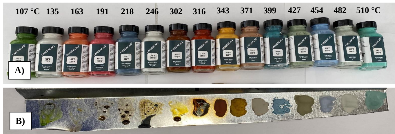
Figure 3.5. Omegalaq™ temperature sensitive paints applied at gradations of approximately 30 °C used to quantify fire temperature. A) Omegalaq™ paints from lowest to highest temperature. B) Example of paint change resulting from heat exposure in a lab setting.
