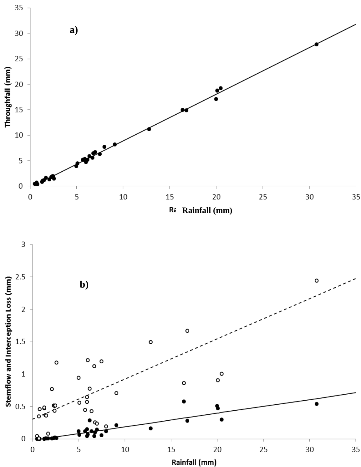
Figure 3.7: a) Event throughfall and b) event stemflow (mm) —●— and interception loss (mm) ---○--- versus rainfall (mm).
