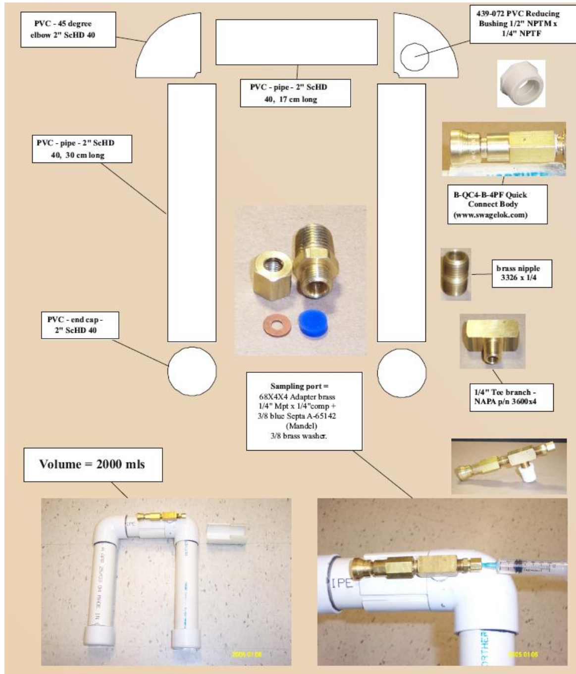
Figure 2.4. Schematic – SPARC PVC Methane collection apparatus (yoke) (Iwaasa et al, 2005).
