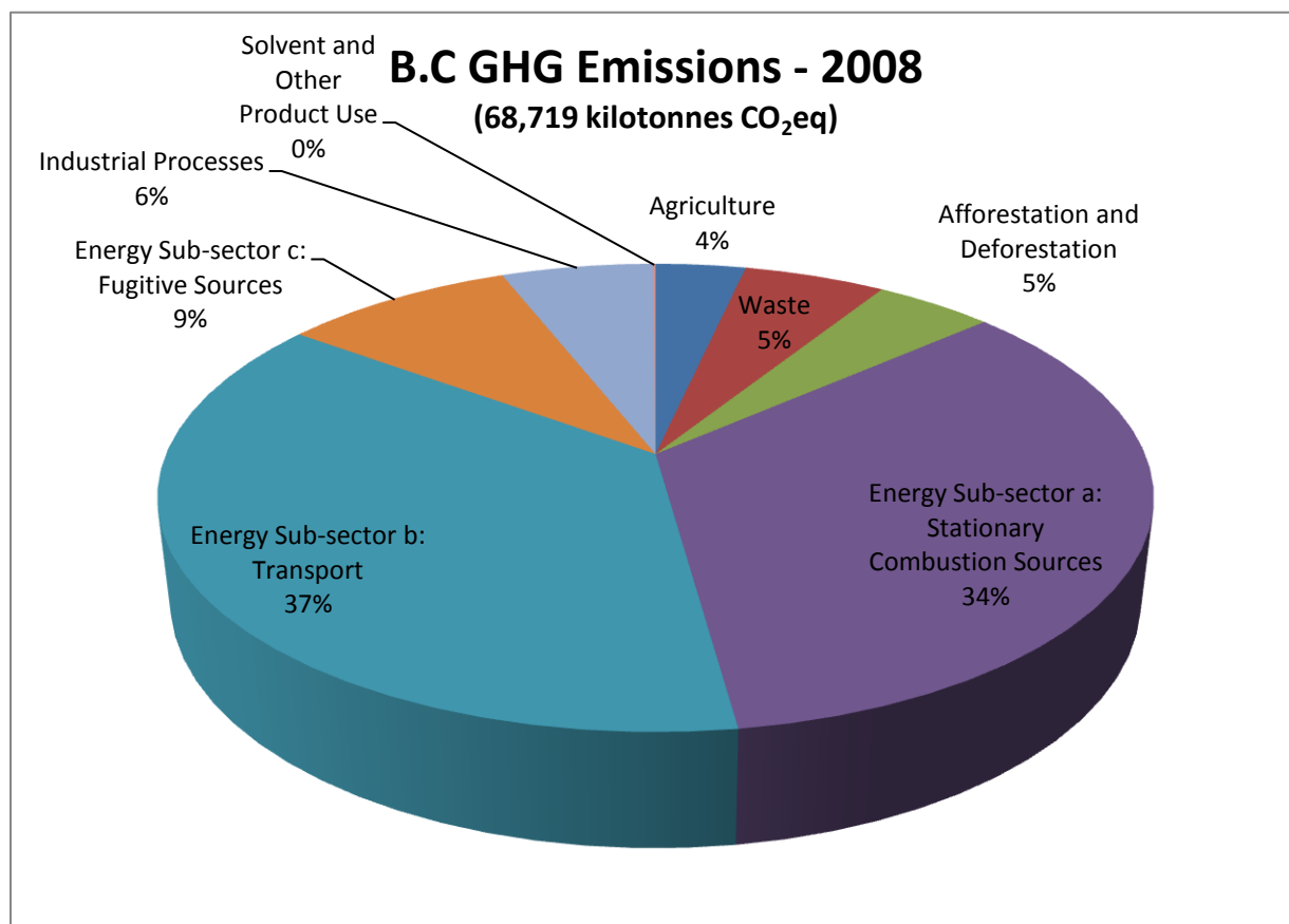
Figure 4.2. B.C. GHG Emissions - 2008. (adapted from BC Ministry of Environment (2010)).
