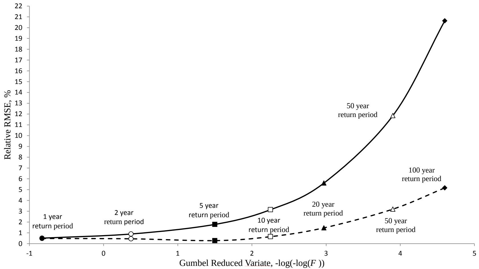
Figure 2.7. 100 Mile House winter maximum daily snowfall relative root mean square errors, RMSEs of estimated quantiles for associated return periods and Gumbel reduced variation of non-exceedance probability, F . Estimation method: at-site (solid line) and regional (dashed line).
