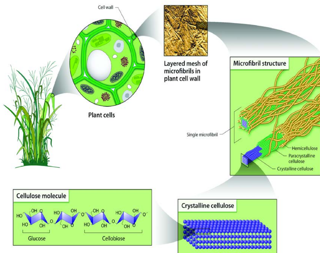
Figure 1.2 Schematic representation of cellulose structure (courtesy of the US Department of Energy Genome Program, available at http://genomics.energy.gov ).
